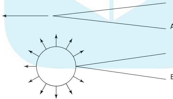
Figure 5-17: (A) The crack tends to go along the same direction if not stopped. (B) Introducing a spherical hole disperses the crack's forces.
